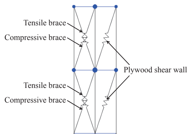
Figure 11: Earthquake response analysis model
