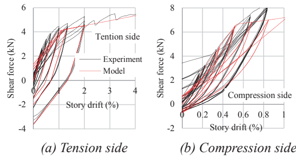
Figure 7: Hysteresis model of braced frame with the new fastener
