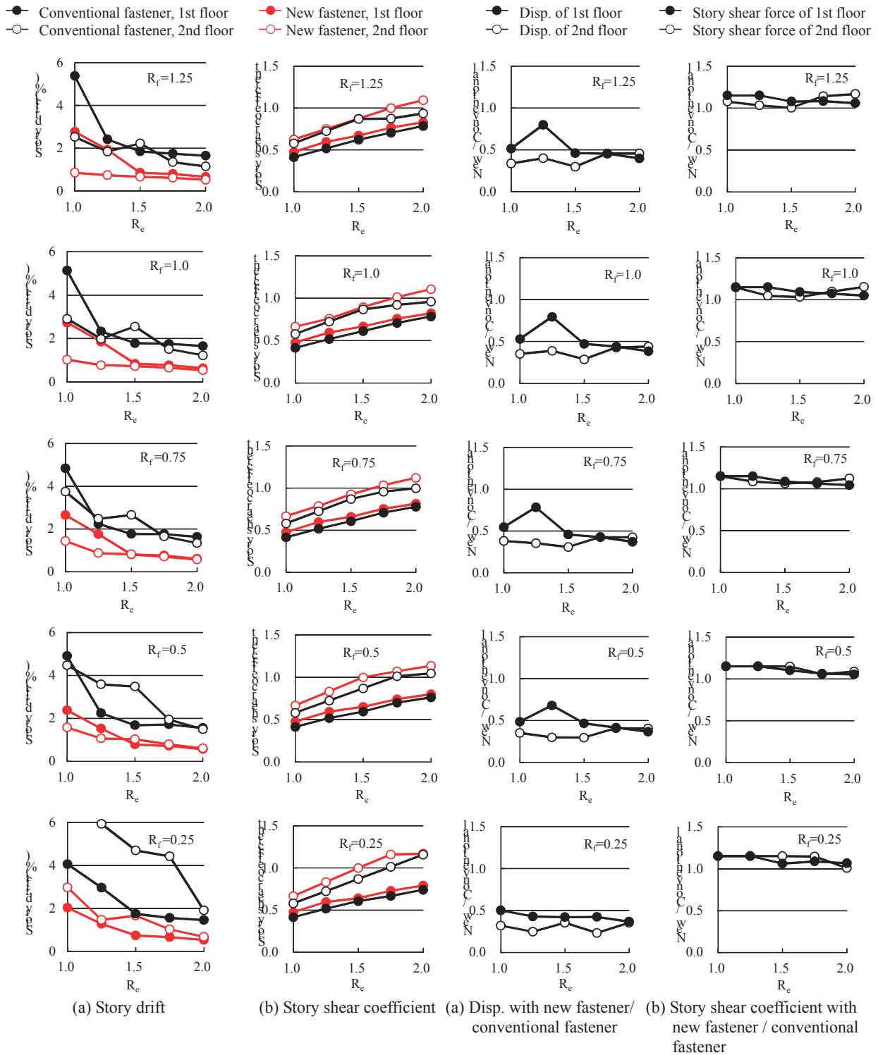
Figure 14: Maximum earthquake response under JMA Kobe wave
