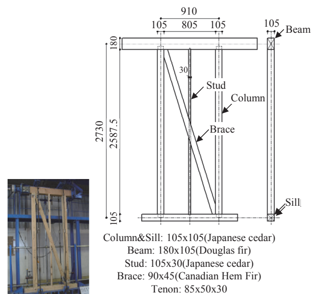
Figure 4: Frame with single brace specimen
