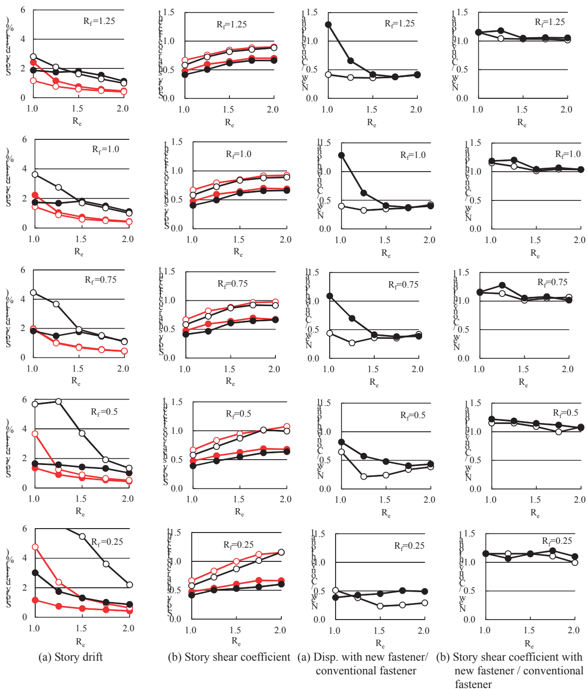
Figure 16: Maximum earthquake response under BCJL2 wave
