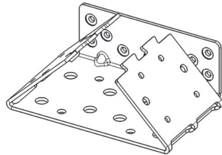
Figure 3: Turning down to form the fastener
