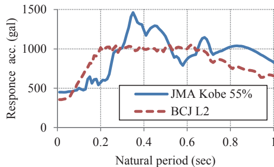
Figure 13: Response spectra ( h=5\% )
