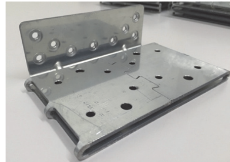
Picture 1: New brace fastener before gluing high damping rubber
