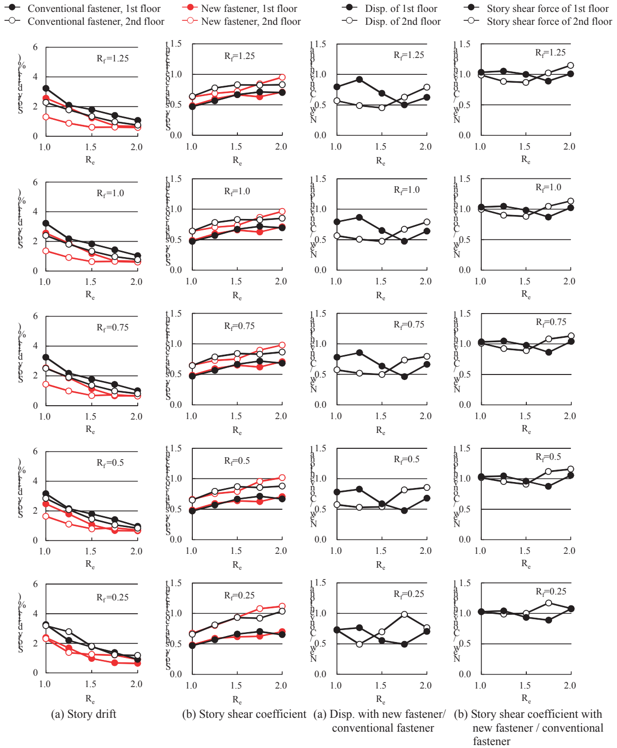
Figure 18: Maximum earthquake response with nailed plywood under JMA Kobe wave
