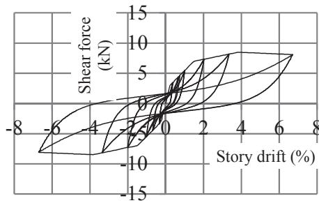
Figure 12: Hysteresis models of frame with nailed plywood
